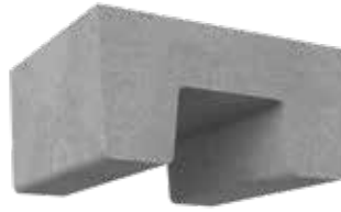
U-BLOCK 350 x 300 x 170 mm
